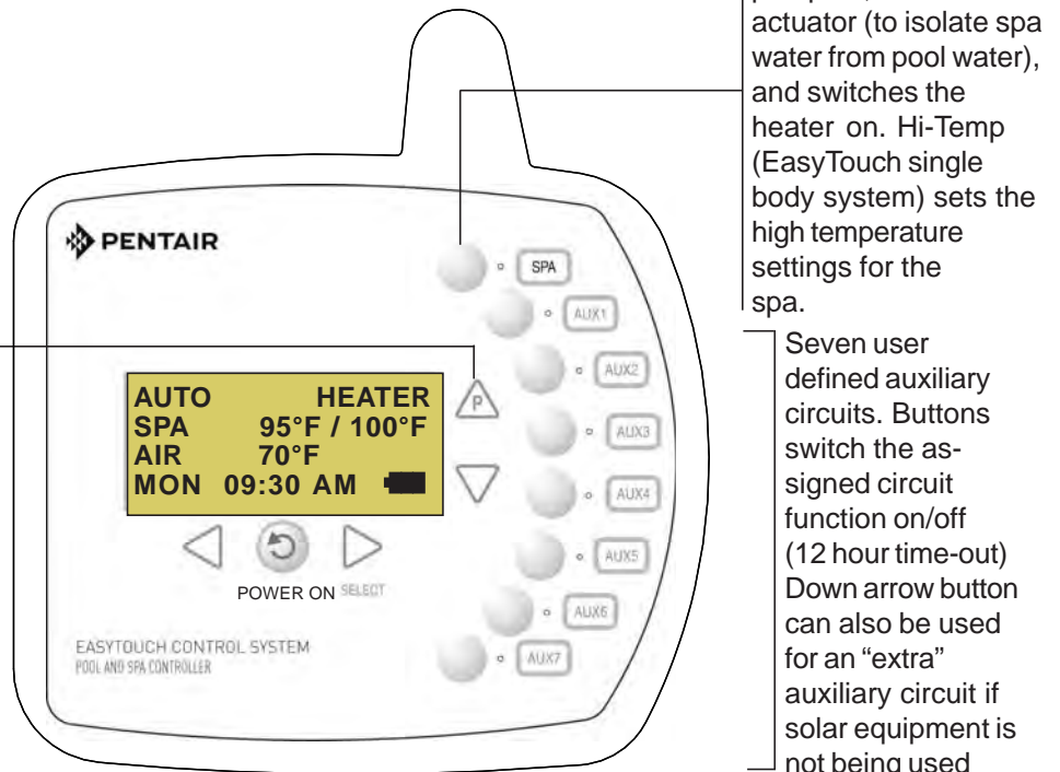
EasyTouch wireless control panel (EasyTouch 8) - (P/N 520547)
